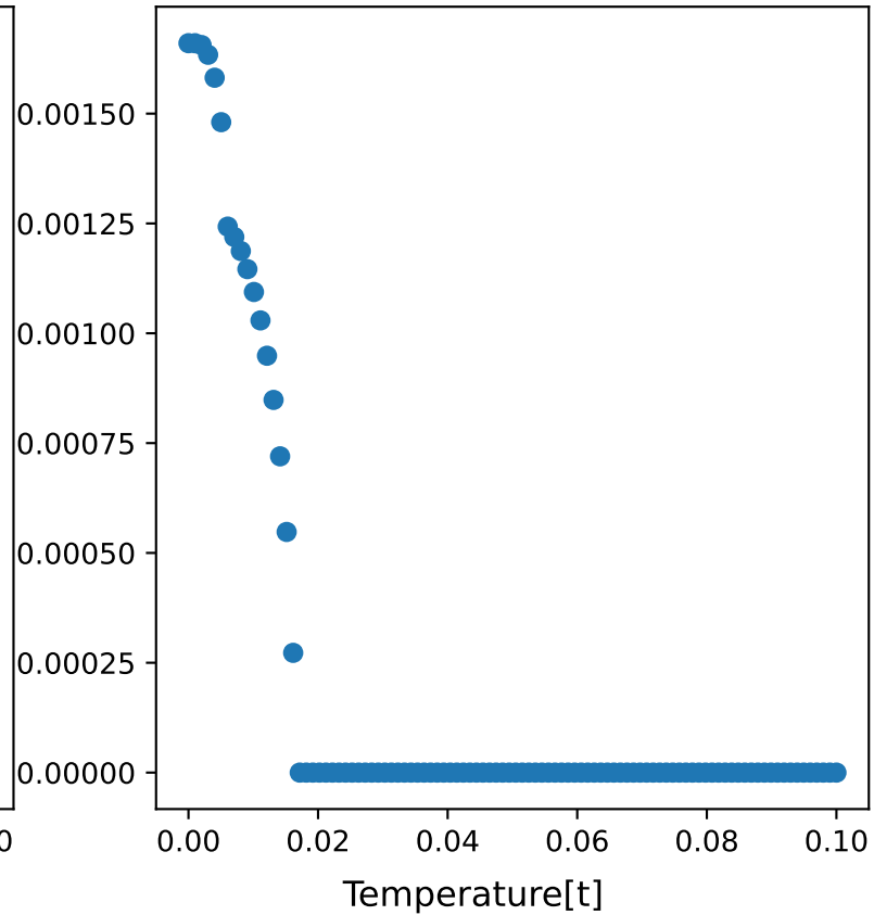
Mean gap
