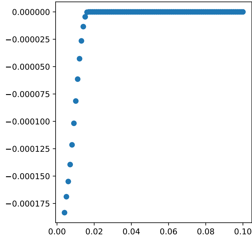
Condensation energy
